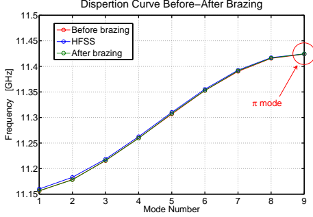
Figure 4: Dispersion curve before and after brazing.
