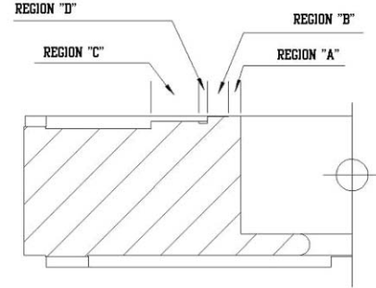
Figure 2: Brazing profile.
