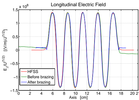
Figure 5: Measured longitudinal electric field on axis.
