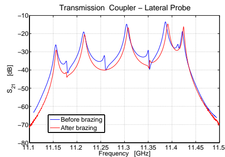
Figure 3: Transmission coefficient between the lateral antenna and the central coupler.
