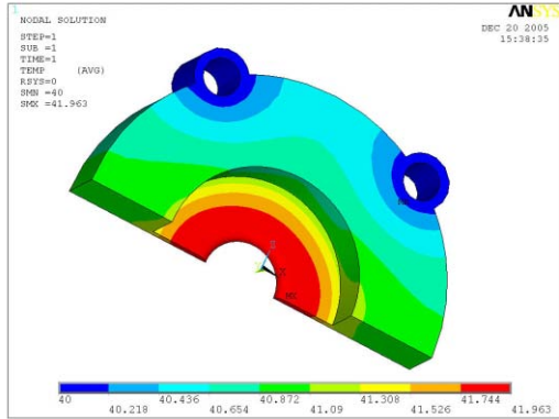
Figure 7: \pi -mode cavity with tubes at 30^\circ working on duty cycle 2 ( 5E - 5 ).
