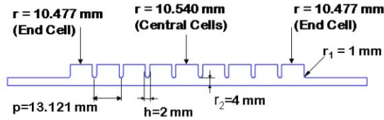
Figure 1: 2D profile of the X-band structure.
