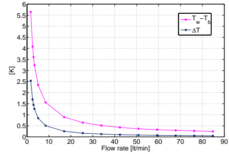
Figure 8: Thermal gradient behaviour in the cooling system.
