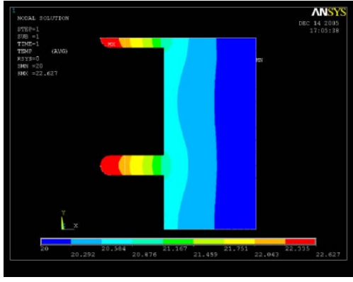
Figure 6: Thermal field in the \pi -mode cavity.
