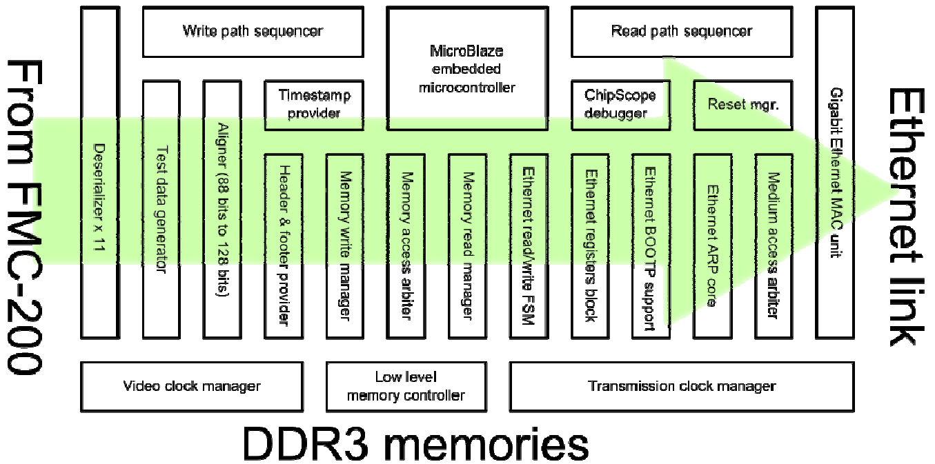
Figure 6. Image Acquisition System FPGA firmware block diagram
