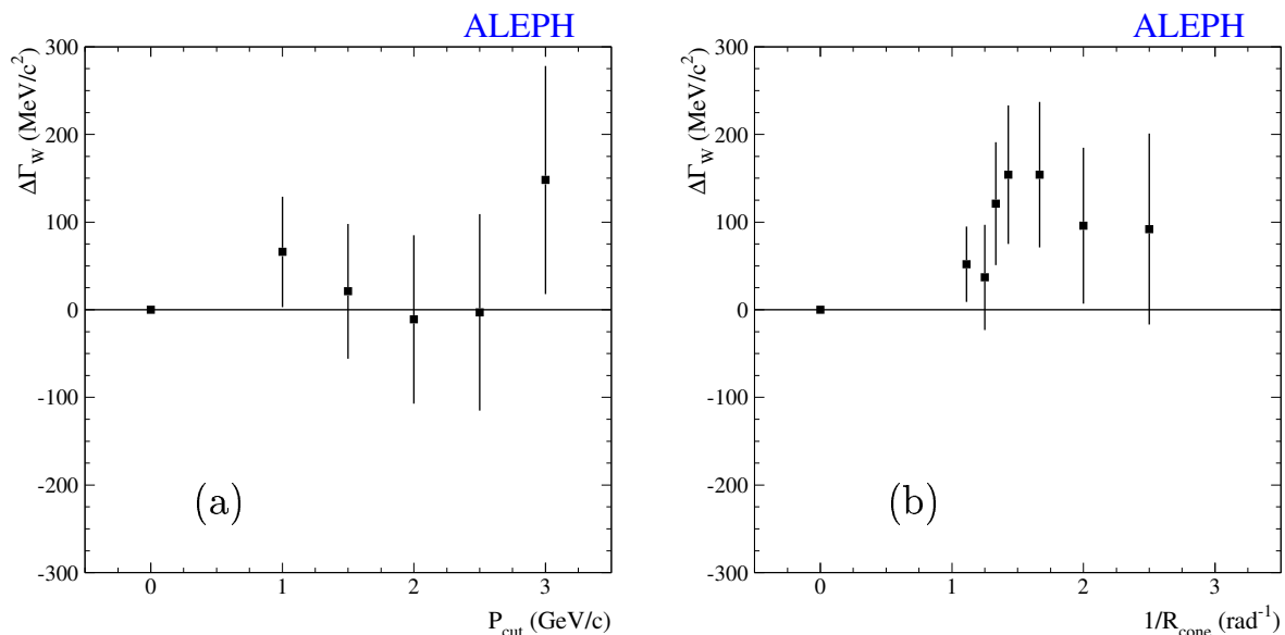
Figure 10: W width differences \Delta\Gamma_W versus (a) PCUT and (b) inverse CONE radius for data from the q\bar{q}q\bar{q} channel. The errors take into account the correlation at each point with the standard analysis.
