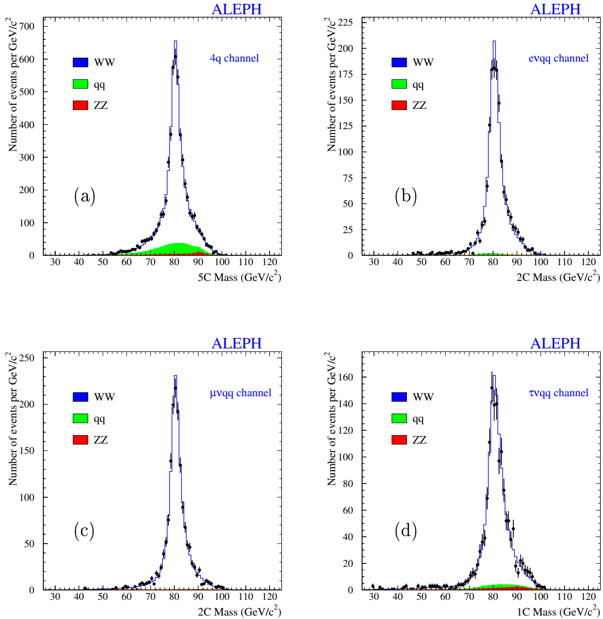
Figure 3: Mass distributions in the: (a) 4q , (b) e\nu q\bar{q} , (c) \mu\nu q\bar{q} and (d) \tau\nu q\bar{q} channels for data (points with error bars), non-WW background (shaded area) and signal+background Monte Carlo with m_W values set to those fitted from each individual channel (solid line histogram). For the 4q channel, the distribution shows the 5C kinematically fitted dijet masses before window cuts are applied. For the \ell\nu q\bar{q} channels, the distributions show the 2C (or 1C) kinematic fits before window cuts.
