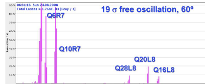
Figure 4: Control room display with losses created by aperture scans in the LHC ARC.
