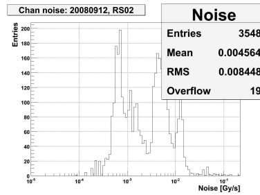
Figure 8: Bias current and noise level distribution of all ionisation chamber beam loss channels in the ring. The upper limit corresponds to the beam permit threshold setting.
