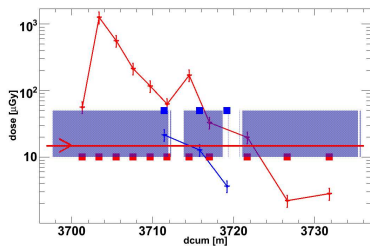
Figure 3: Beam loss measurements showing the loss which initiated the second quench of an LHC magnet. The red and blue curves show the measurements initiated by the same impacting protons on either side of the magnet.
