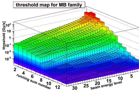
Figure 6: Beam permit threshold settings of a bending magnet channel as function of the beam energy level (lowest beam energy level corresponds to 250 GeV) and running sum window (lowest corresponds to 40 \mu\text{s} and largest to 80 s).
