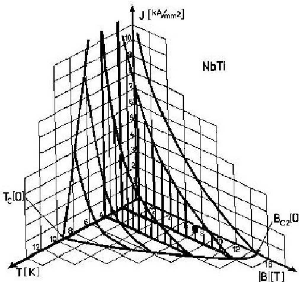
Figure 1.5: Superconducting phase diagram of the NbTi.
