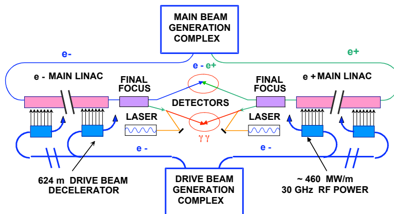
Fig. 1: Overall layout of the CLIC complex.
