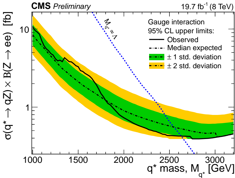
(a) Gauge interaction production
