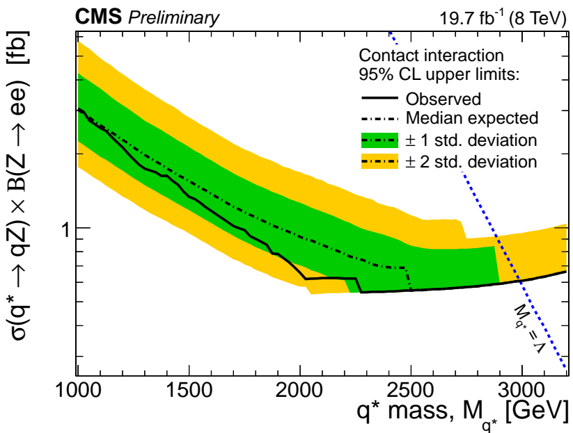
(b) Contact interaction production
