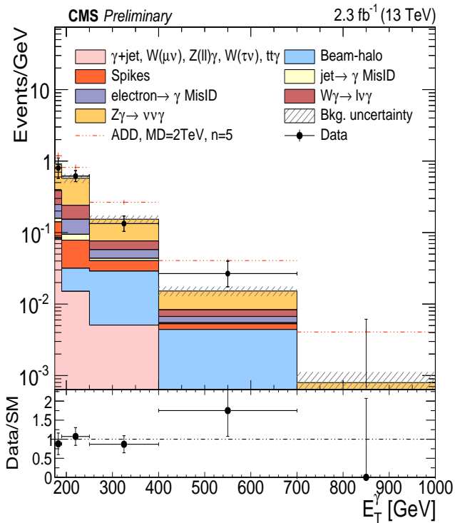
(a) Photon p_T
