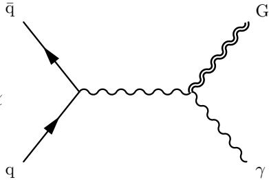
(c) ADD graviton production.
