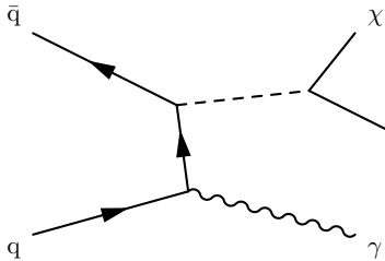
(a) DM simplified model.
