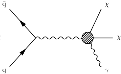
(b) Electroweak-DM effective interaction.
