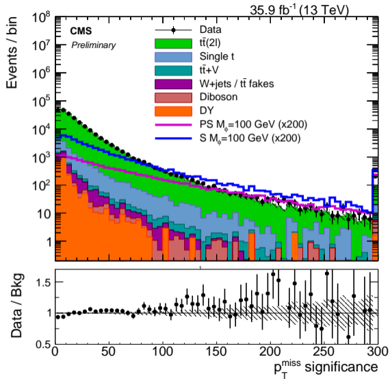
(a) p_T^{\text{miss}} significance
