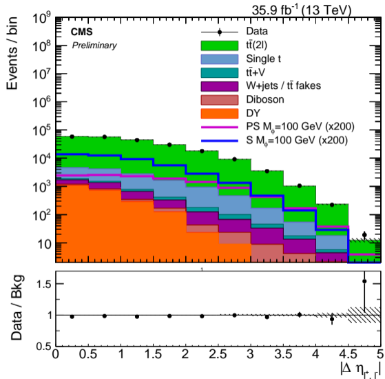
(a) |\Delta\eta(\ell\ell)|
