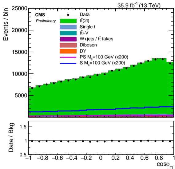
(b) \cos\Phi_{\ell\ell}
