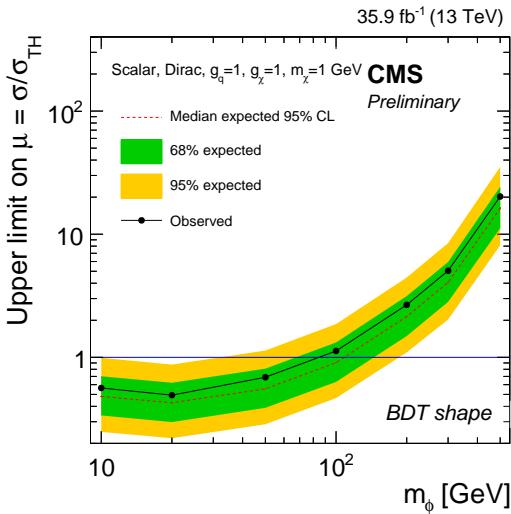
(c) BDT discriminant: scalar mediator
