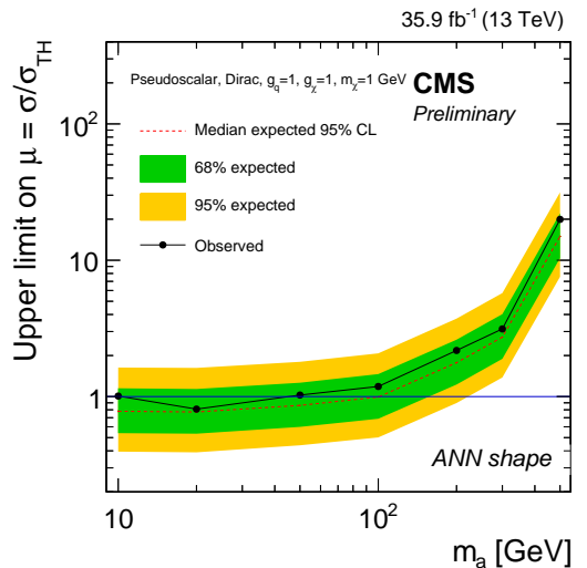
(f) ANN discriminant: pseudoscalar mediator
