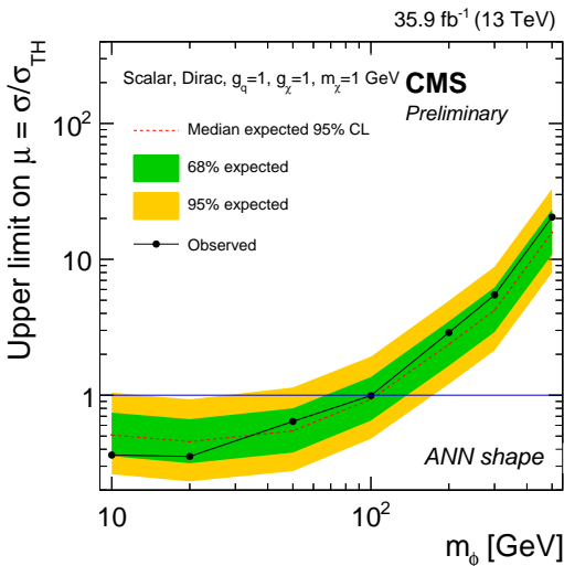
(e) ANN discriminant: scalar mediator
