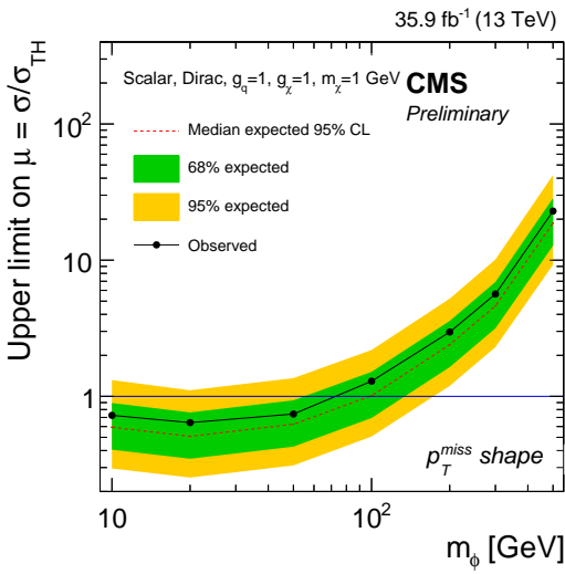
(a) p_T^{\text{miss}} shape: scalar mediator
