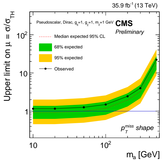
(b) p_T^{\text{miss}} shape: pseudoscalar mediator
