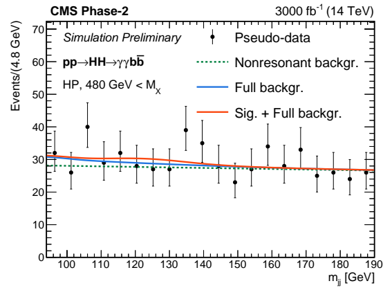
(b) m_{jj} , high mass category
