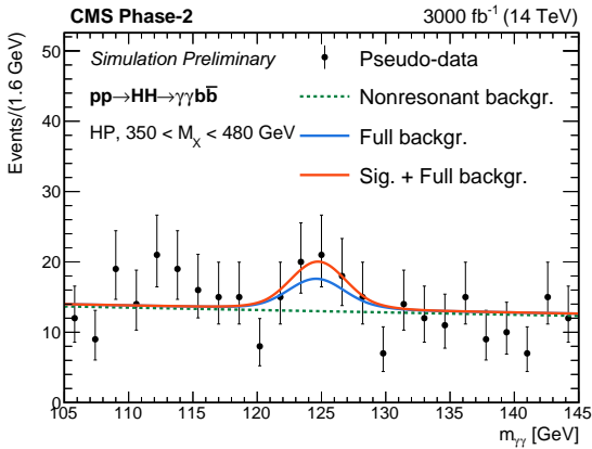
(c) m_{\gamma\gamma} , medium mass category
