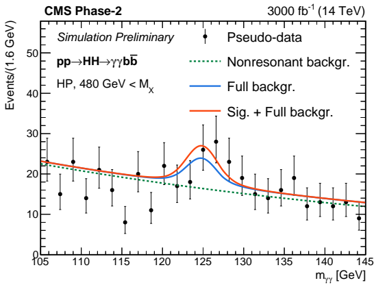
(a) m_{\gamma\gamma} , high mass category
