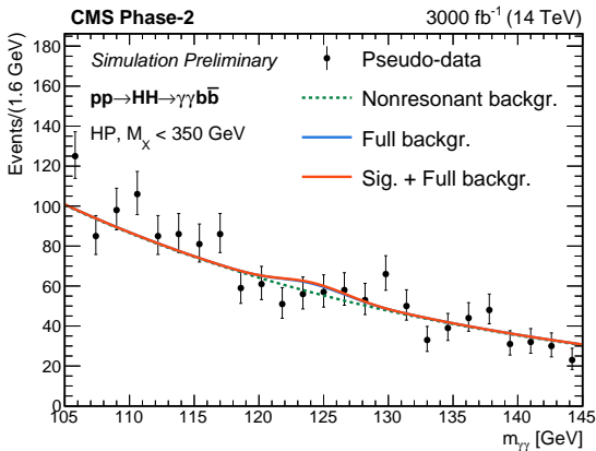
(e) m_{\gamma\gamma} , low mass category
