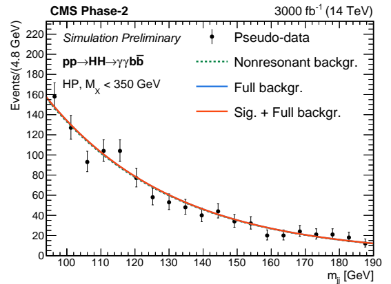
(f) m_{jj} , low mass category
