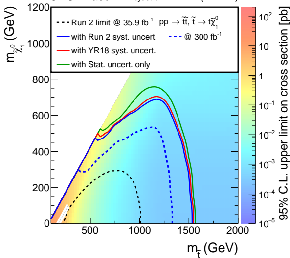
CMS Phase-2 Projection 3 ab -1 (14 TeV)
