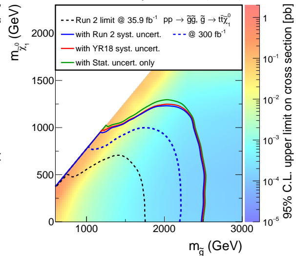
CMS Phase-2 Projection 3 ab -1 (14 TeV)
