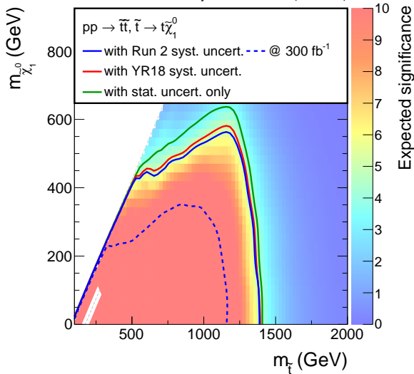
CMS Phase-2 Projection 3 ab -1 (14 TeV)
