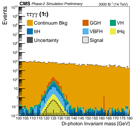
(b) One tau final state
