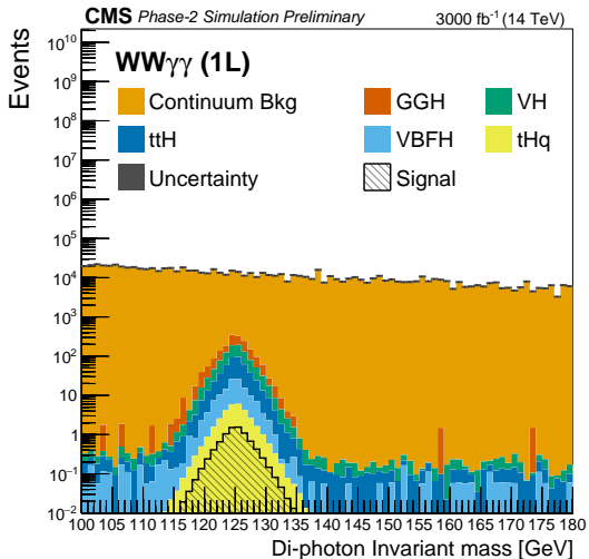
(a) One lepton final state
