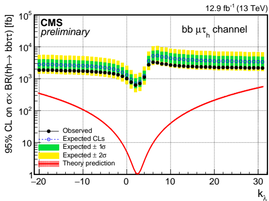
(a) bb\mu\tau_h
