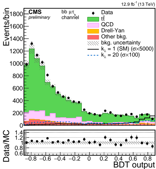
(a) bb\mu\tau_h
