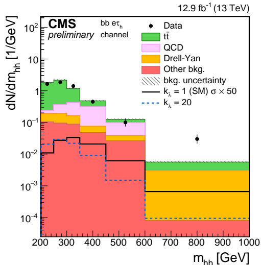
(b) bb e \tau_h
