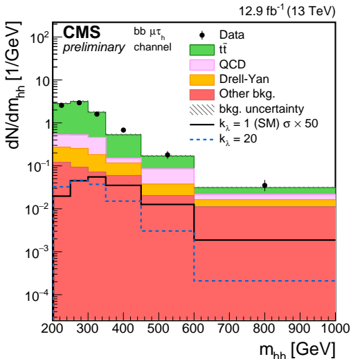
(a) bb \mu \tau_h
