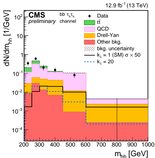
(c) bb \tau_h \tau_h
