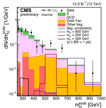
(f) \tau_h\tau_h : resolved 2b
