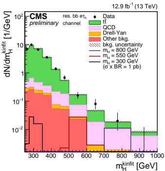
(e) e\tau_h : resolved 2b
