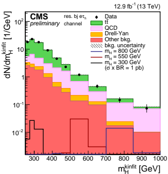
(b) e\tau_h : resolved 1jet-1b
