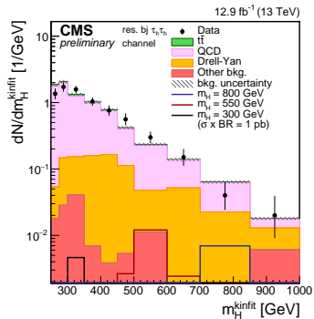
(c) \tau_h\tau_h : resolved 1jet-1b
