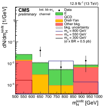
(h) e\tau_h : boosted
