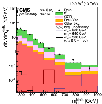
(a) \mu\tau_h : resolved 1jet-1b
