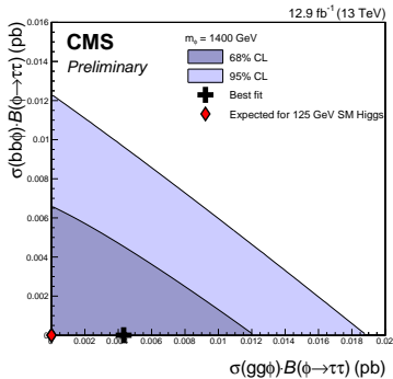
(a) m_\phi = 1400 GeV
