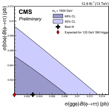
(b) m_\phi = 1800 GeV
