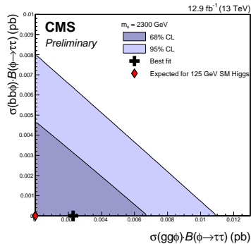
(c) m_\phi = 2300 GeV
