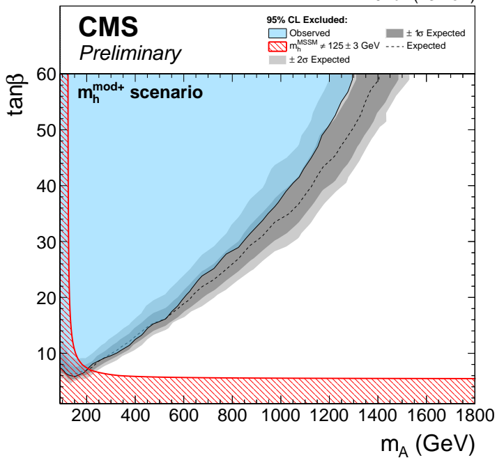
(a) m_h^{\text{mod+}}
