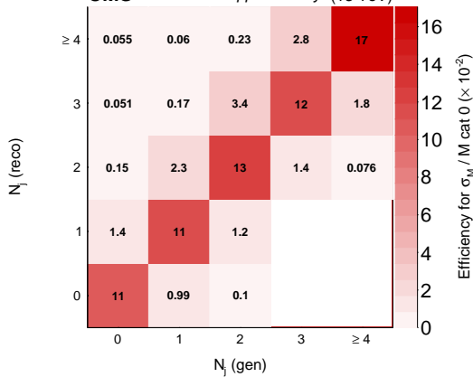
CMS Simulation Supplementary (13 TeV)
