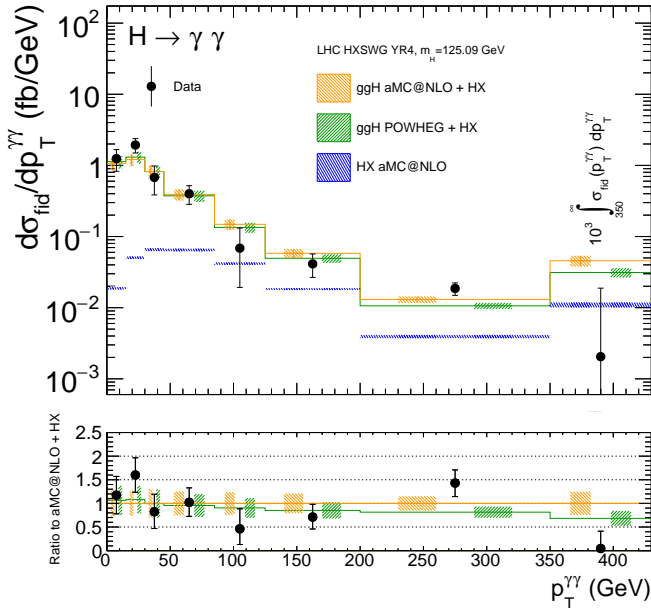
(a) p_{T,\gamma\gamma} differential cross-section
