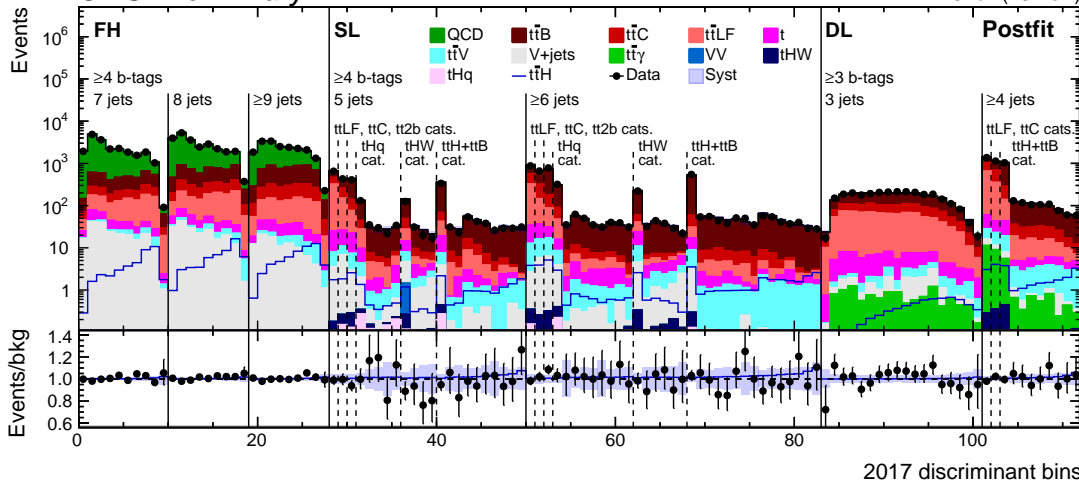
2017 discriminant bins
