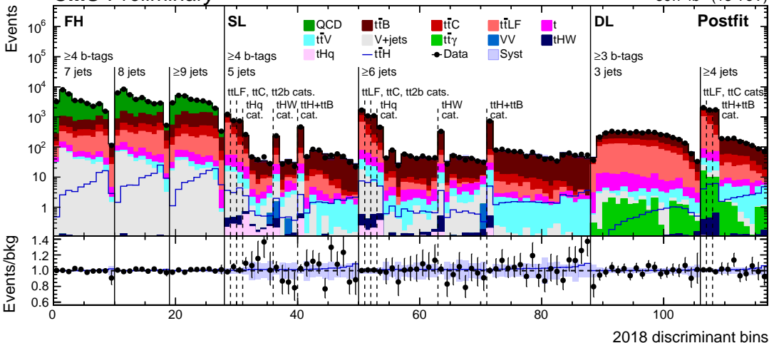
2018 discriminant bins
