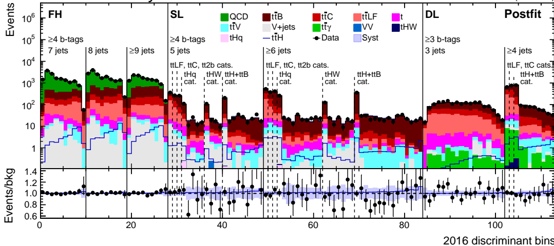
2016 discriminant bins
