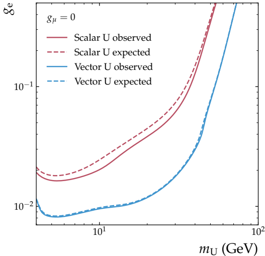
CMS preliminary 19.7 fb -1 (8 TeV) + 138 fb -1 (13 TeV)
