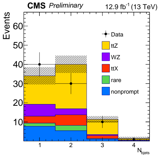
(b) Number of b-tagged jets
