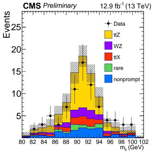
(a) Di-lepton invariant mass
