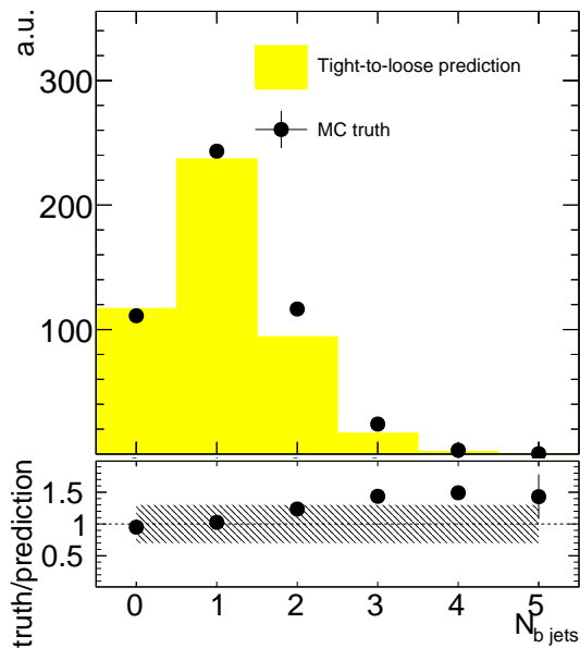
CMS Simulation
