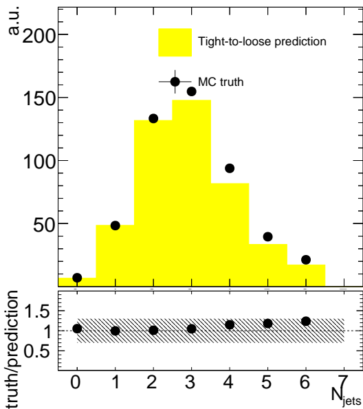
CMS Simulation
