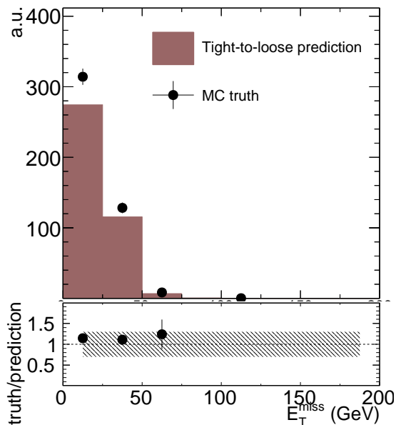
CMS Simulation
