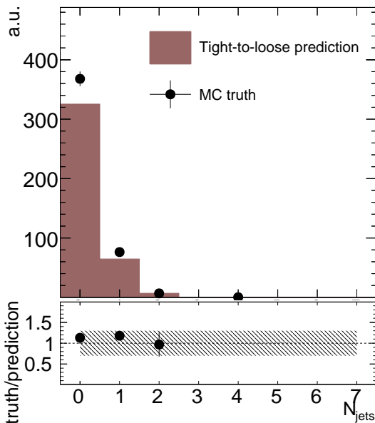
CMS Simulation
