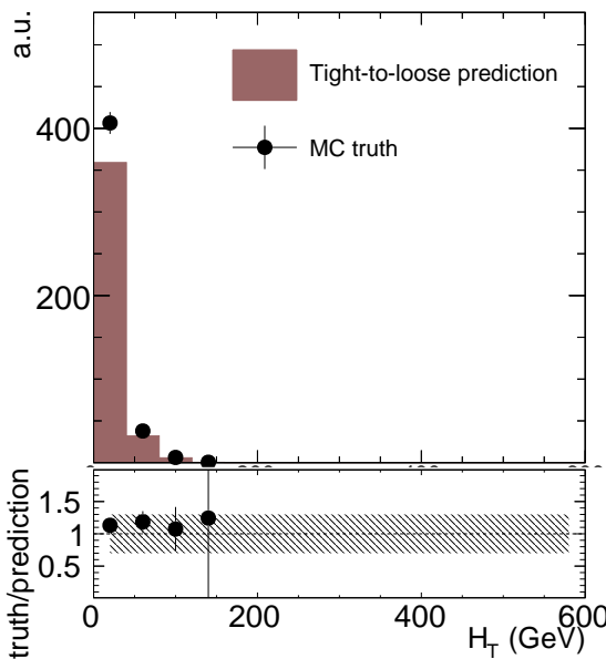
CMS Simulation
