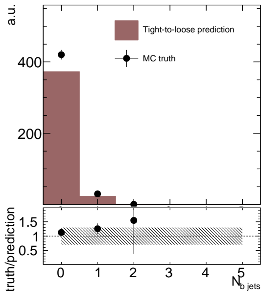
CMS Simulation
