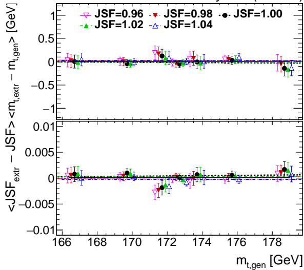
CMS Simulation Preliminary (13 TeV)
