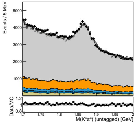
CMS Preliminary 35.9 fb -1 (13 TeV)
