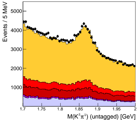
CMS Preliminary 35.9 fb -1 (13 TeV)
