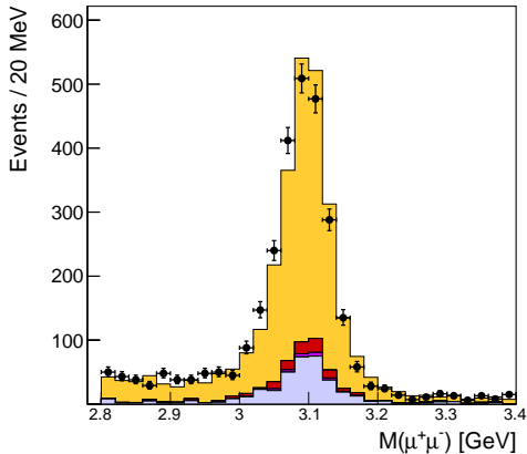
CMS Preliminary 35.9 fb -1 (13 TeV)
