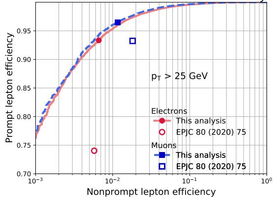
CMS Simulation Preliminary
