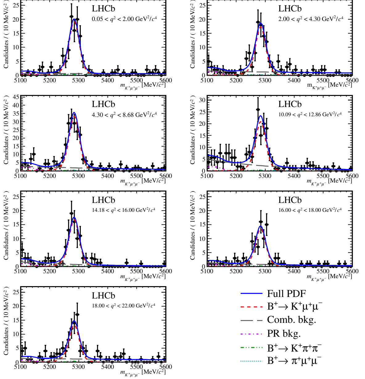
Figure 1: Invariant m_{K\mu\mu} distributions for B^+ \rightarrow K^+\mu^+\mu^- decays in the q^2 seven bins used in the analysis.
