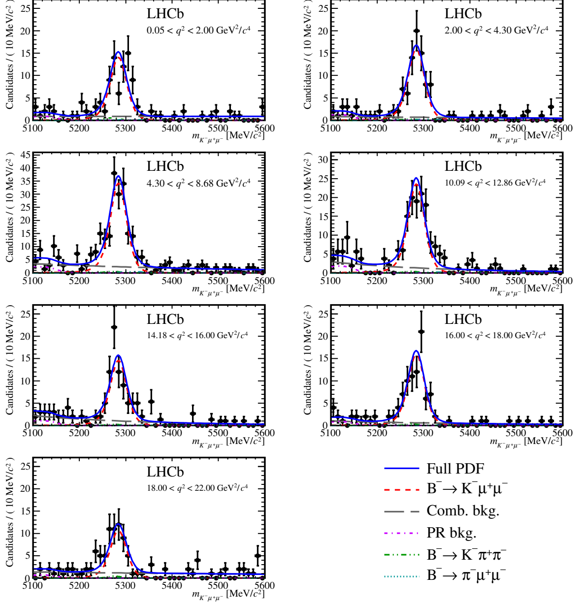
Figure 2: Invariant m_{K\mu\mu} distributions for B^- \rightarrow K^- \mu^+ \mu^- decays in the seven q^2 bins used in the analysis.
