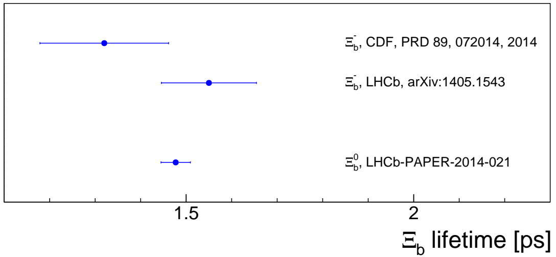
Figure 7: Lifetime measurements of the \Xi_b^- baryon and the \Xi_b^0 lifetime as determined in this analysis.
