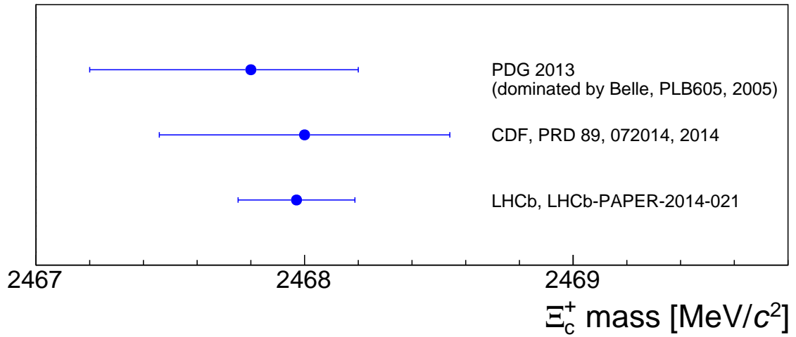
Figure 6: Summary of mass measurements of the \Xi_c^+ baryon. The PDG result is the average of several results, but is dominated by the indicated Belle measurement.
