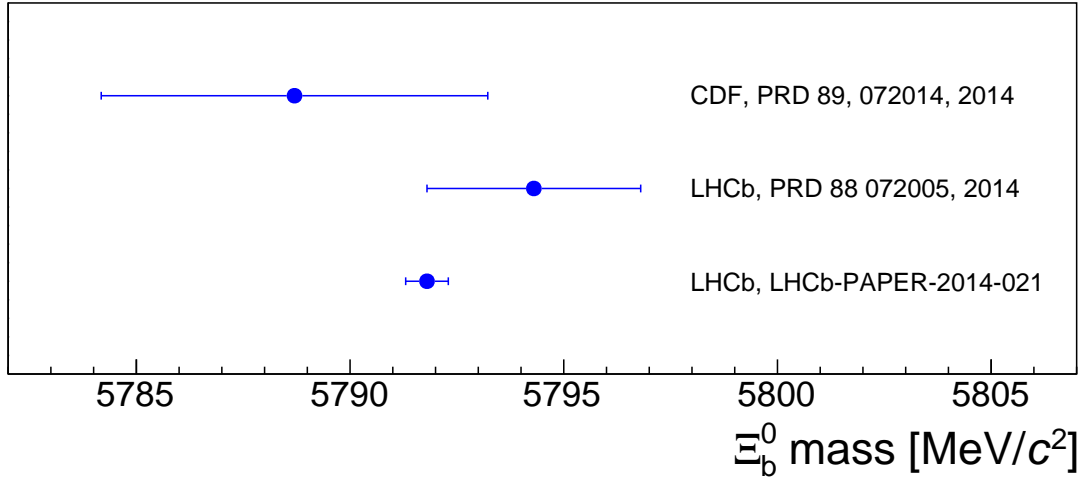
Figure 5: Summary of mass measurements of the \Xi_b^0 baryon.
