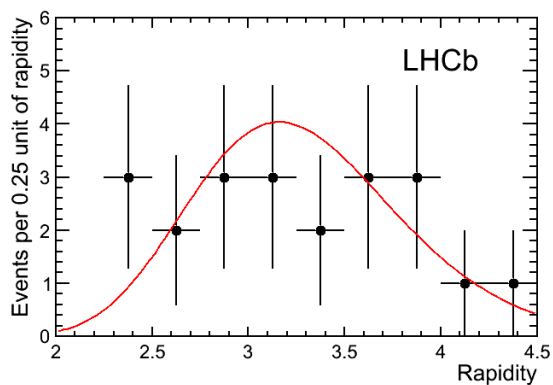
Figure 1: Rapidity of J/\psi candidates with p_T^2 < 1 \text{ GeV}^2 compared to the acceptance-corrected rapidities for the Durham model.
