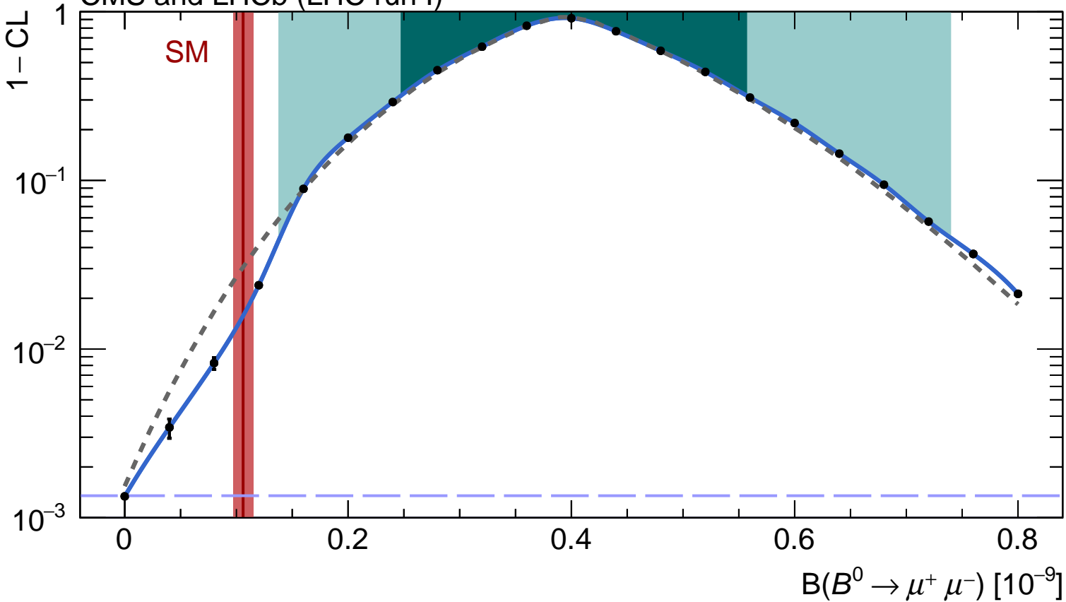
CMS and LHCb (LHC run I)
