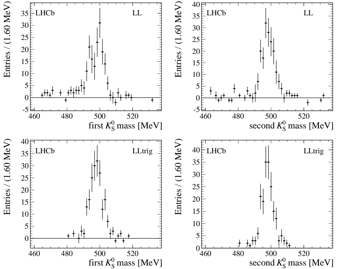
Figure 1: Invariant mass of the K_S^0 candidates in the signal, background subtracted, in (top) LL, and (bottom) LLtrig. The first K_S^0 candidate is the one with the larger p_T .
