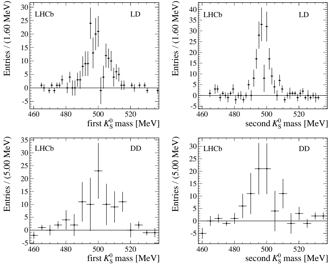
Figure 2: Invariant mass of the K_S^0 candidates in the signal, background subtracted, in (top) LD, and (bottom) DD. The first K_S^0 candidate is the one with the larger p_T , except for the case of LD, where the first K_S^0 candidate is the long one.
