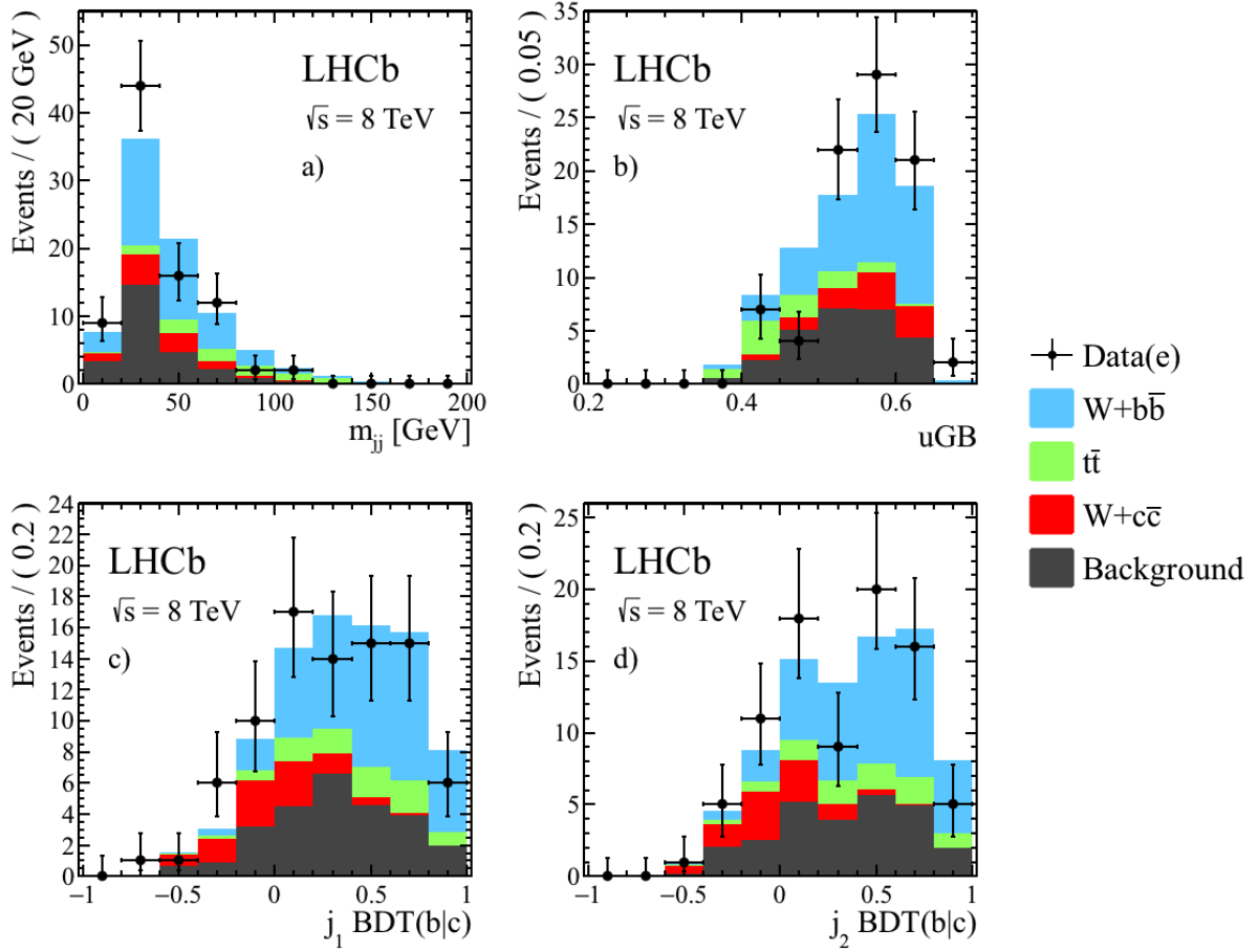
Figure 2: Projections of the simultaneous 4D-fit results for the e sample: a) the dijet mass; b) the uGB response; the BDT( b|c ) of the c) leading and d) sub-leading jets.
