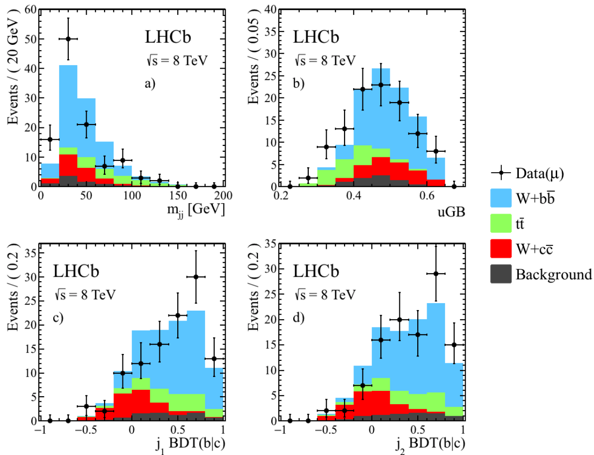
Figure 1: Projections of the simultaneous 4D-fit results for the \mu sample: a) the dijet mass; b) the uGB response; the BDT( b|c ) of the c) leading and d) sub-leading jets.
