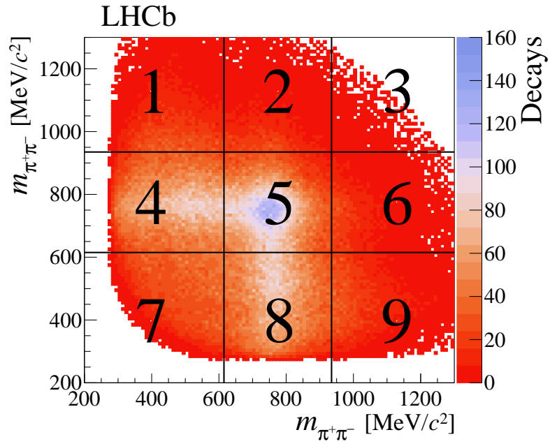
Figure 1: Distribution of candidates in the data in the plane spanned by the invariant masses m_{\pi^+\pi^-} of the two oppositely charged two-pion combinations. The distribution is symmetric by construction. The vertical and horizontal lines illustrate the sector boundaries.
