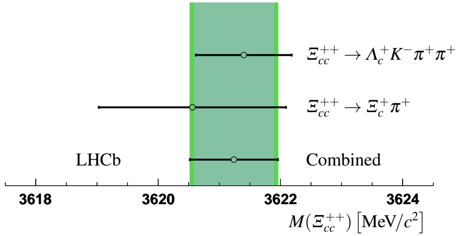
Figure 1: Measured \Xi_{cc}^{++} masses obtained with the decay modes \Xi_{cc}^{++} \rightarrow \Lambda_c^+ K^- \pi^+ \pi^+ and \Xi_{cc}^{++} \rightarrow \Xi_c^+ \pi^+ , and the combined result. The darker green band represents the statistical uncertainty on the combination, and the lighter green band represents the total uncertainty on the combination.
