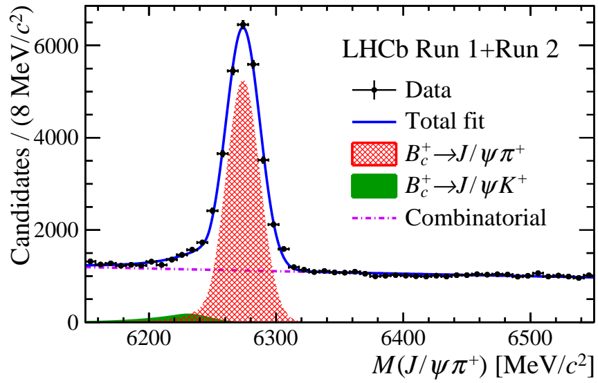
Figure 1: Invariant mass distribution of the selected B_c^+ candidates in the whole p_T range. The fit results are overlaid.
