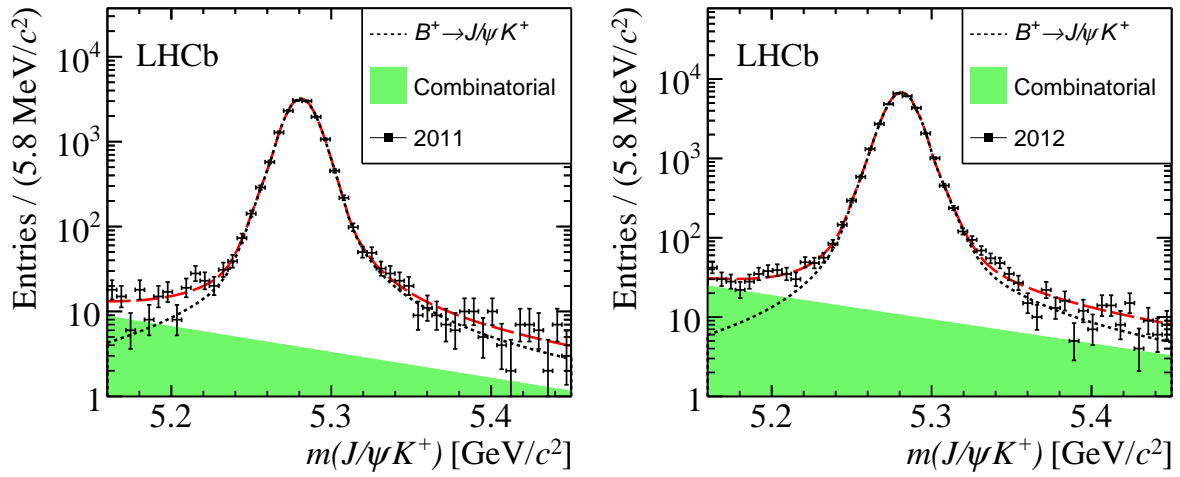
Figure 1: Distribution of m(J/\psi K^+) in the (left) 2011 and (right) 2012 data sets. Overlaid are the fit results.
