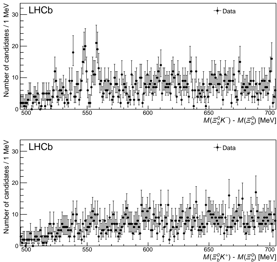
Figure 1: Distribution of the mass difference for (top) right-sign \Xi_b^0 K^- candidates, and (bottom) \Xi_b^0 K^+ wrong-sign candidates.
