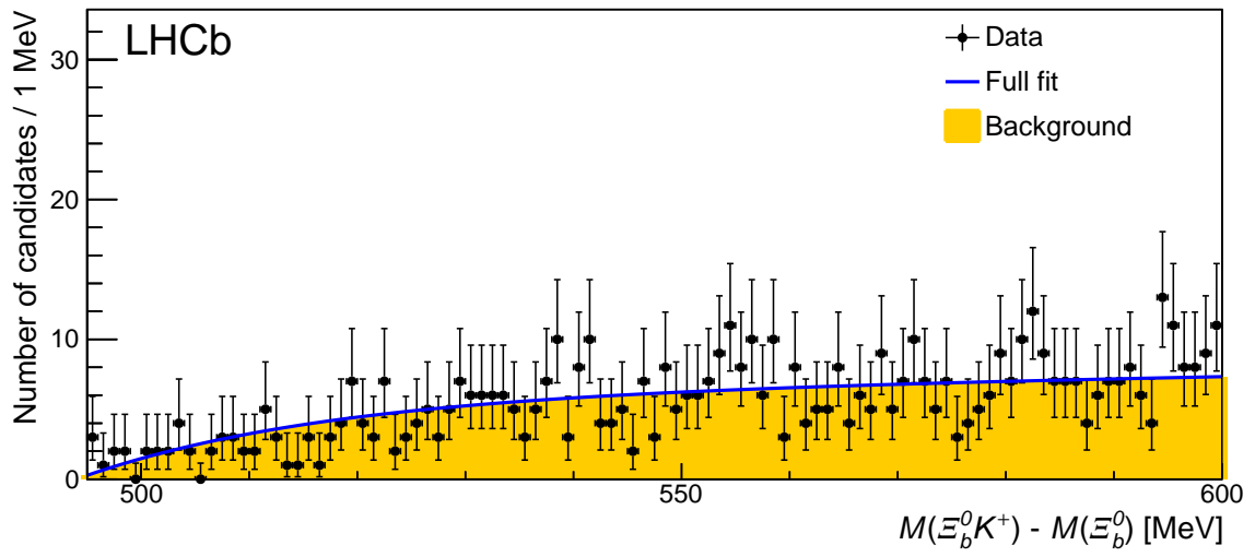
Figure 2: Distribution of the mass difference for (top) right-sign \Xi_b^0 K^- candidates, and (bottom) \Xi_b^0 K^+ wrong-sign candidates, zoomed into the signal region. The results of the fit are shown.
