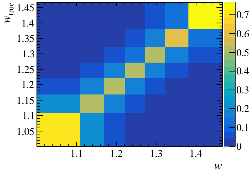
Figure 2: Migration matrix of w and w_{\text{true}} .
