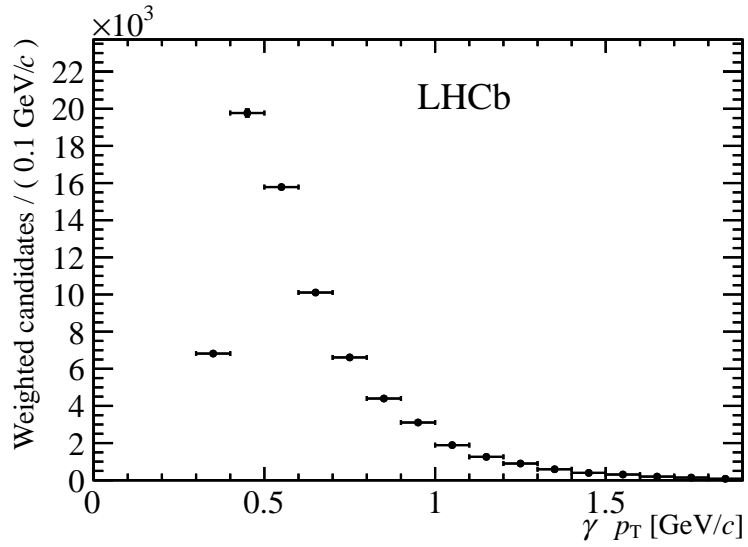
Figure 1: Distribution of the reconstructed photon p_T .
