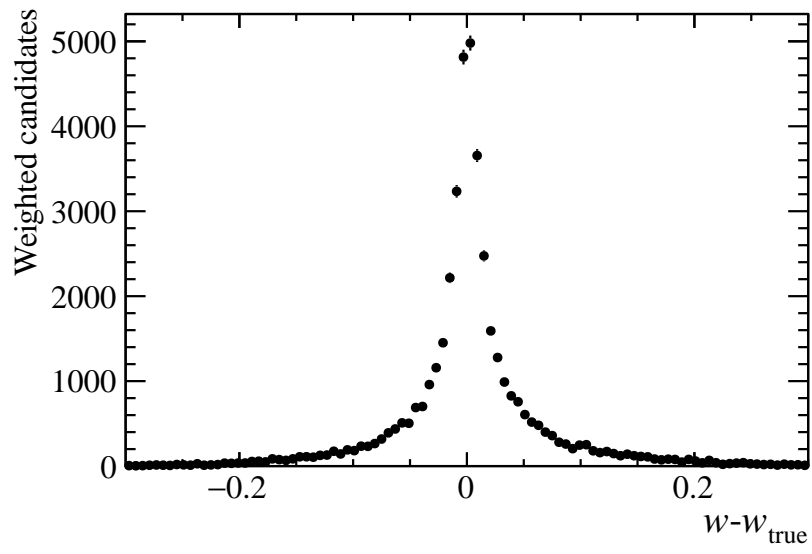
Figure 3: Resolution on the w variable.
