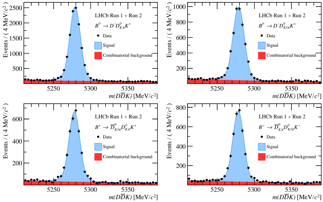
Figure 2: Fits to the invariant-mass distribution of all studied B \rightarrow D\bar{D}K modes
