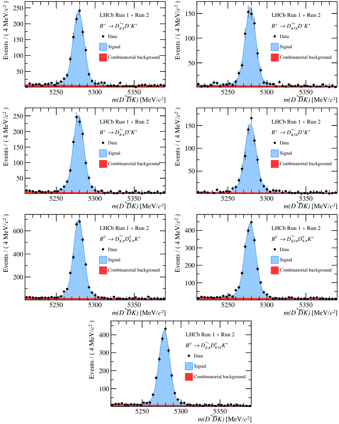
Figure 1: Fits to the invariant-mass distribution of all studied B \rightarrow D^* \bar{D} K modes
