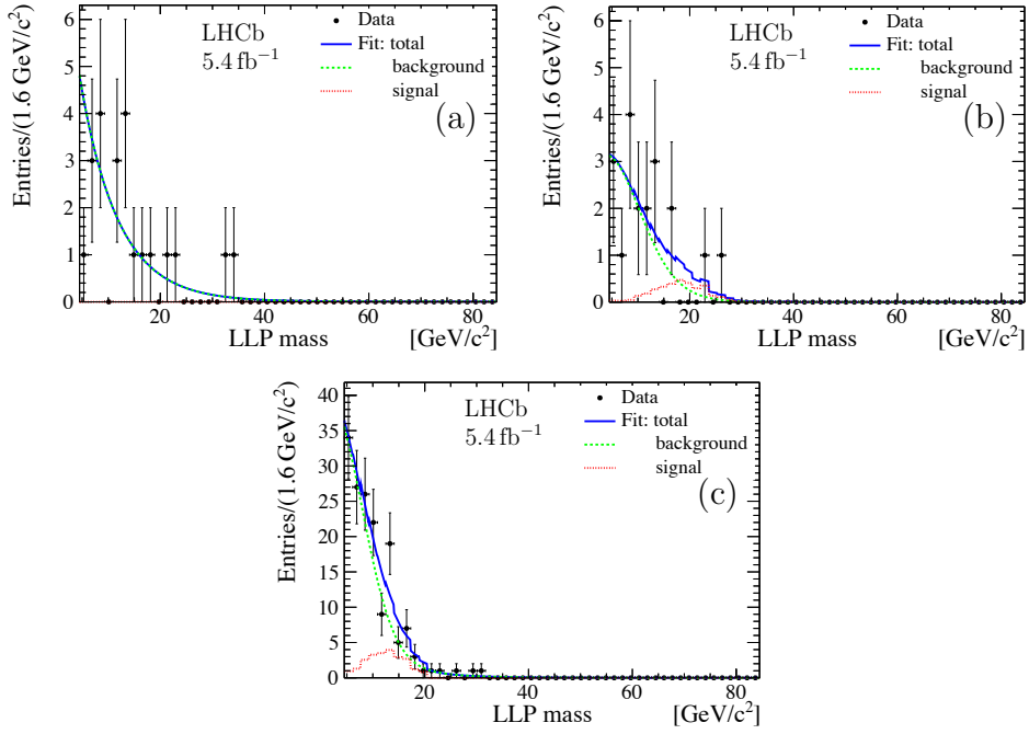
Figure 8: Reconstructed invariant mass of the LLP candidates, with the results of the fits, assuming the theoretical hypotheses: (a): h80-chi30-10ps, (b): chi30-10ps, and (c): h200-chi20-10ps.
