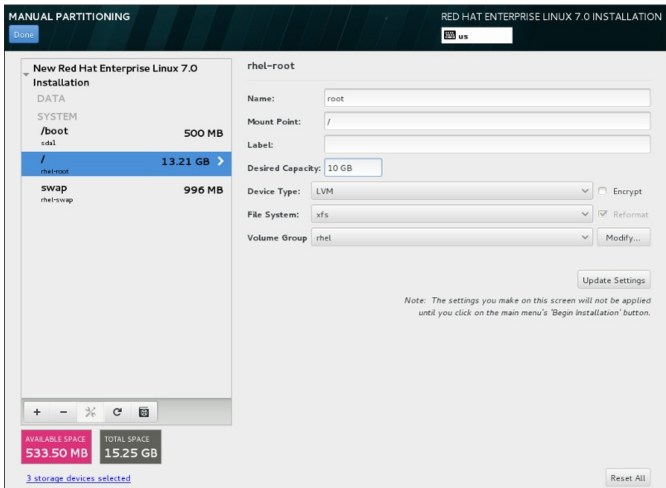
Figure 15.22. Customizing Partitions
