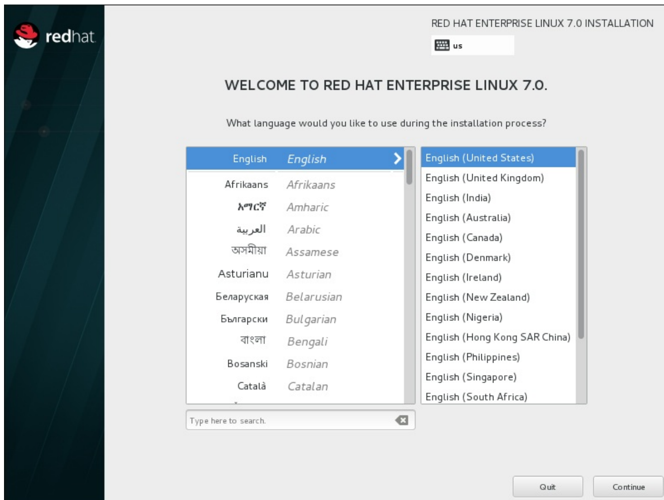
Figure 6.4. Language Configuration
