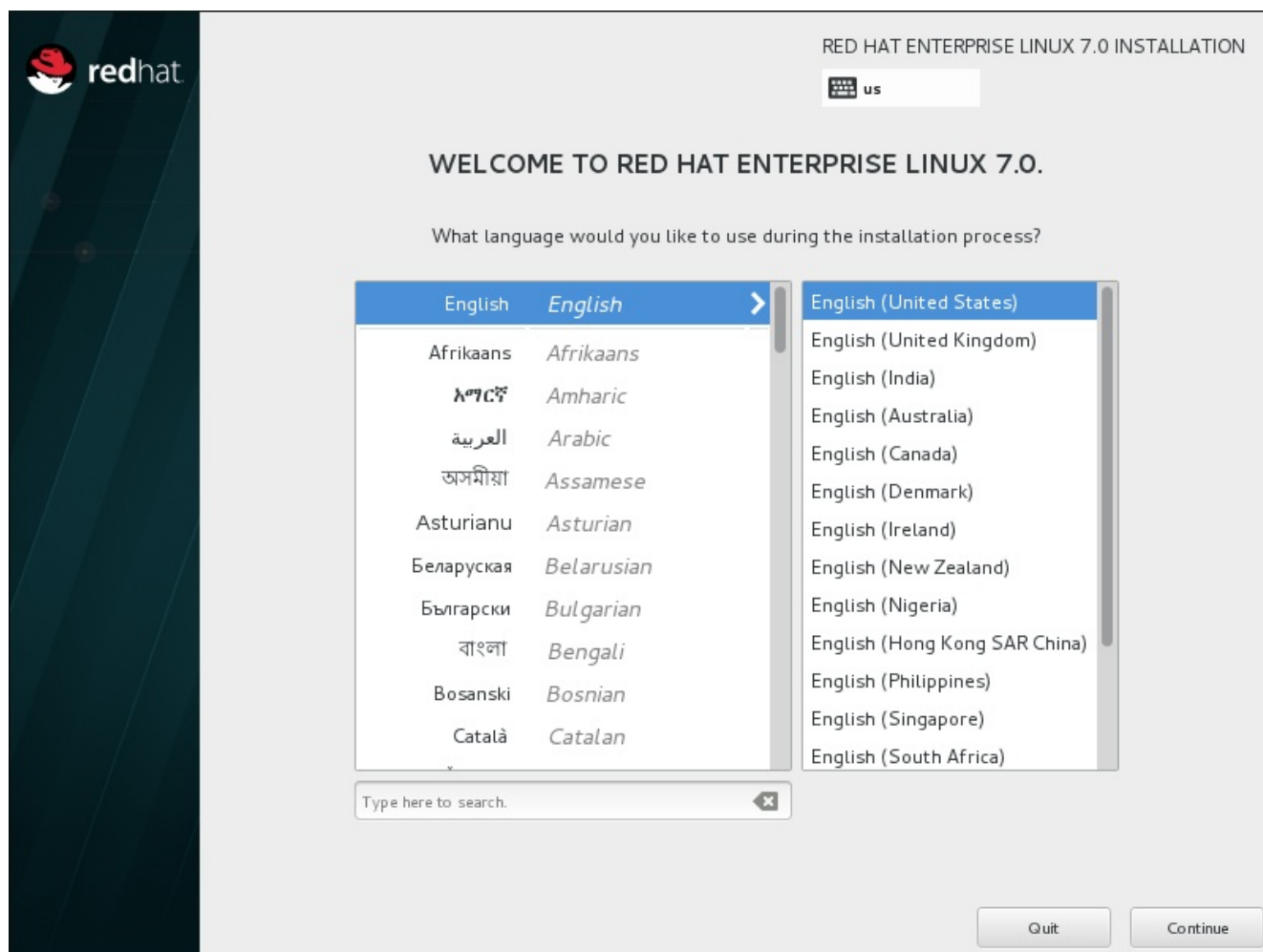
Figure 15.4. Language Configuration
