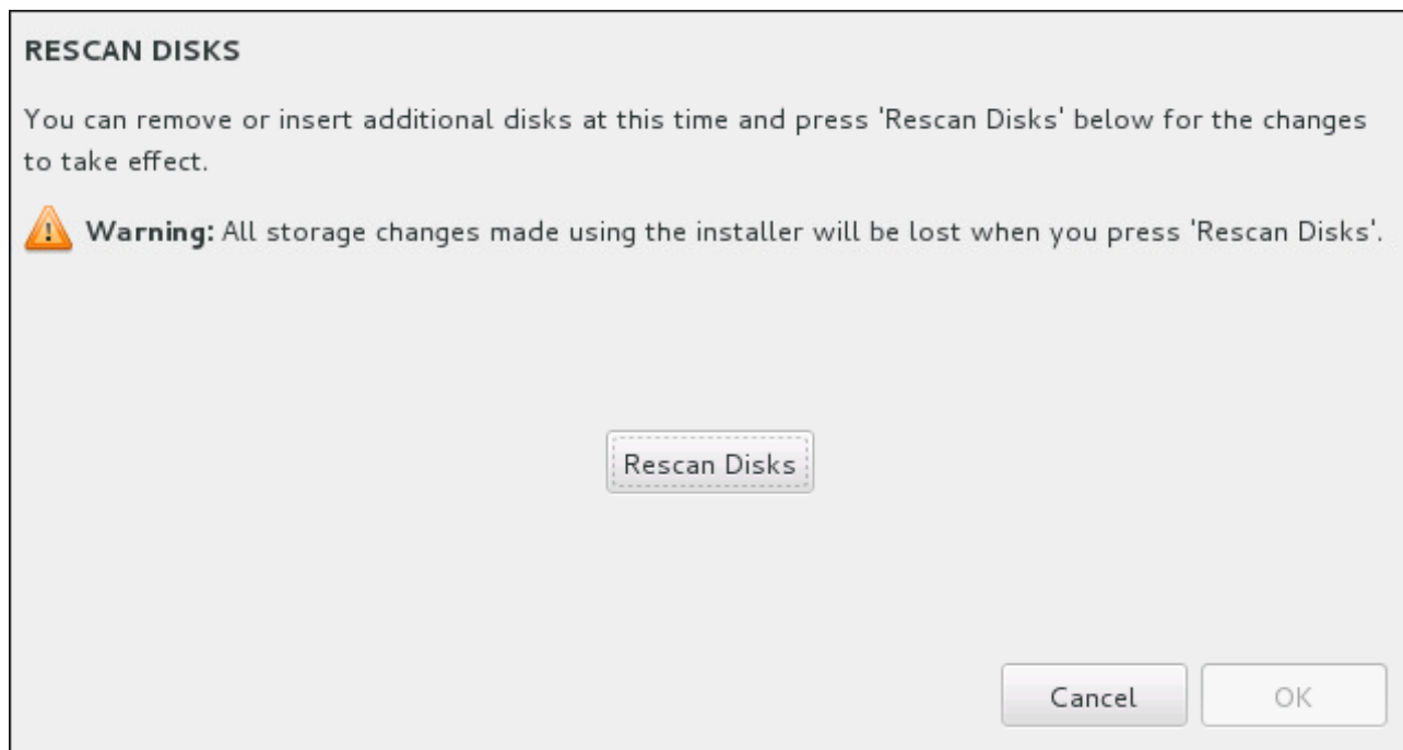
Figure 15.21. Rescanning Disks
