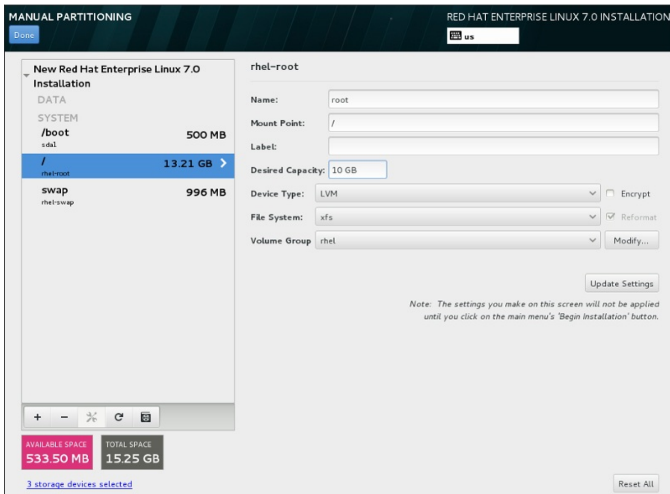
Figure 11.26. Customizing Partitions
