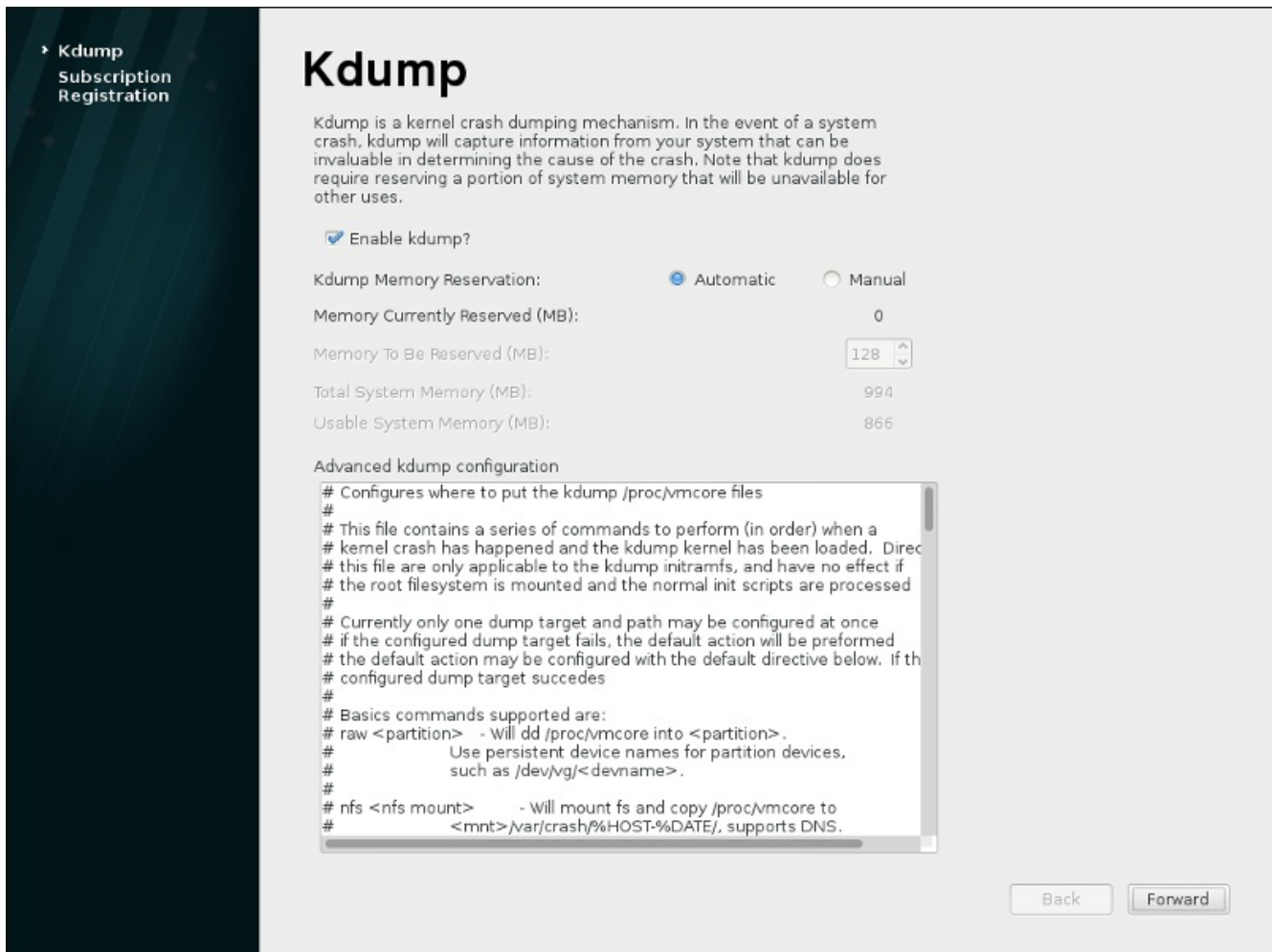
Figure 26.4. Kdump Enabled
