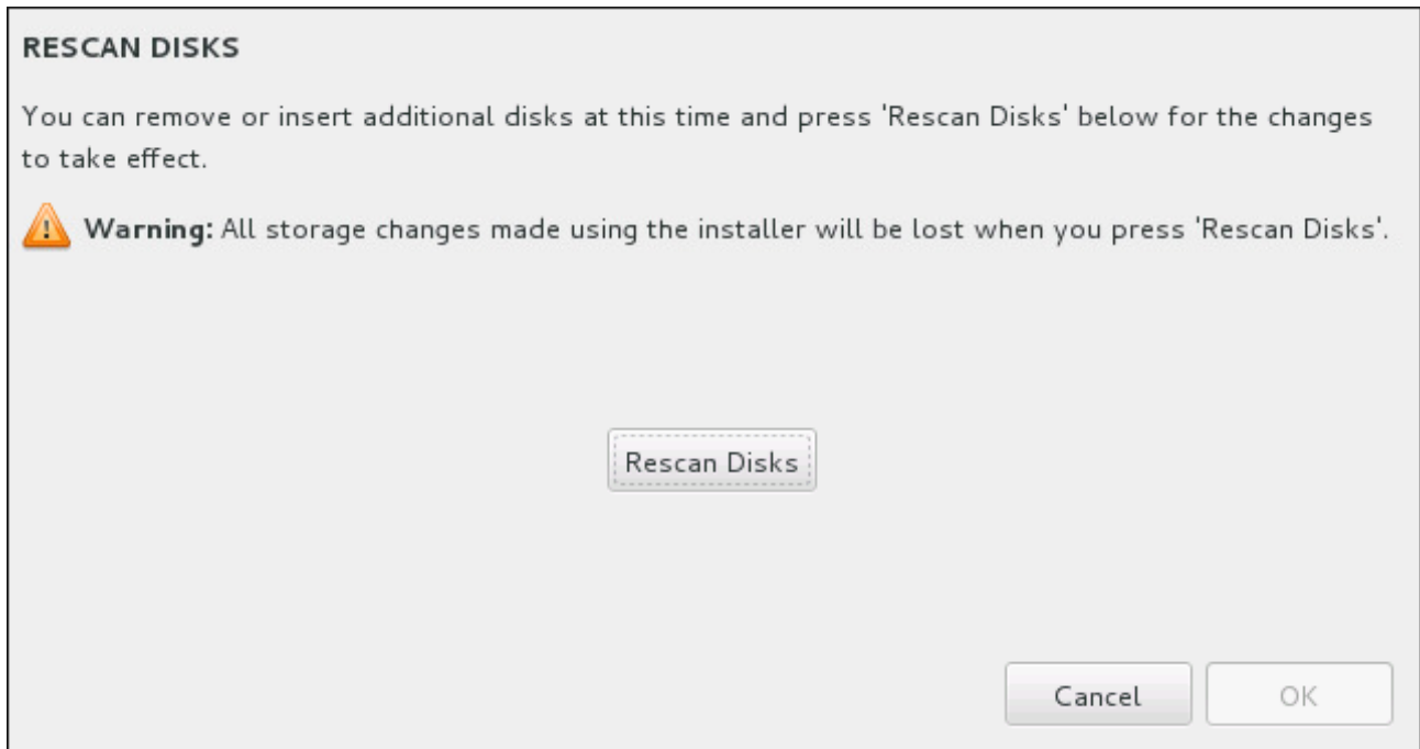
Figure 11.25. Rescanning Disks
