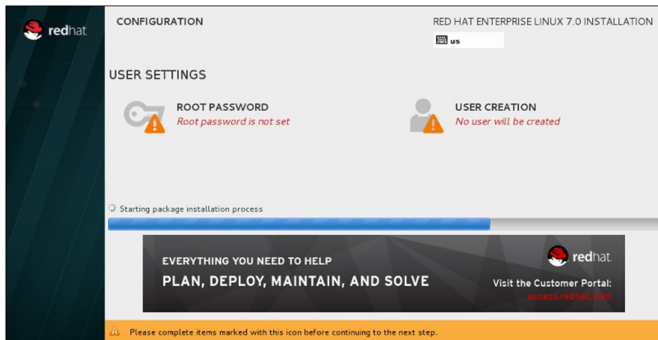
Figure 15.37. Installing Packages
