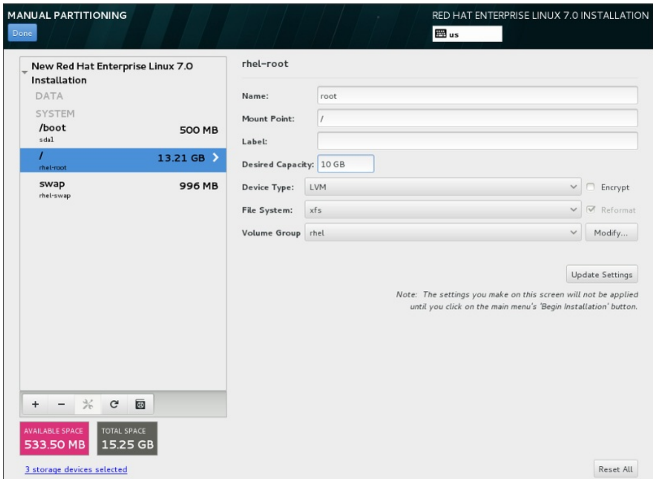
Figure 6.26. Customizing Partitions
