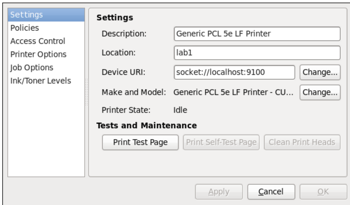
Figure 12.12. Settings page
