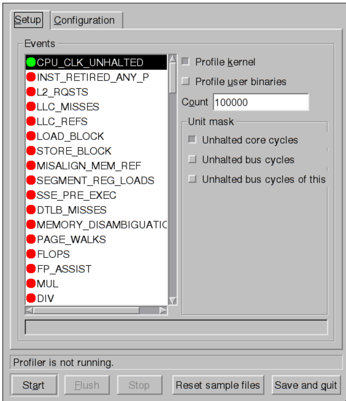
Figure 21.1. OProfile Setup
