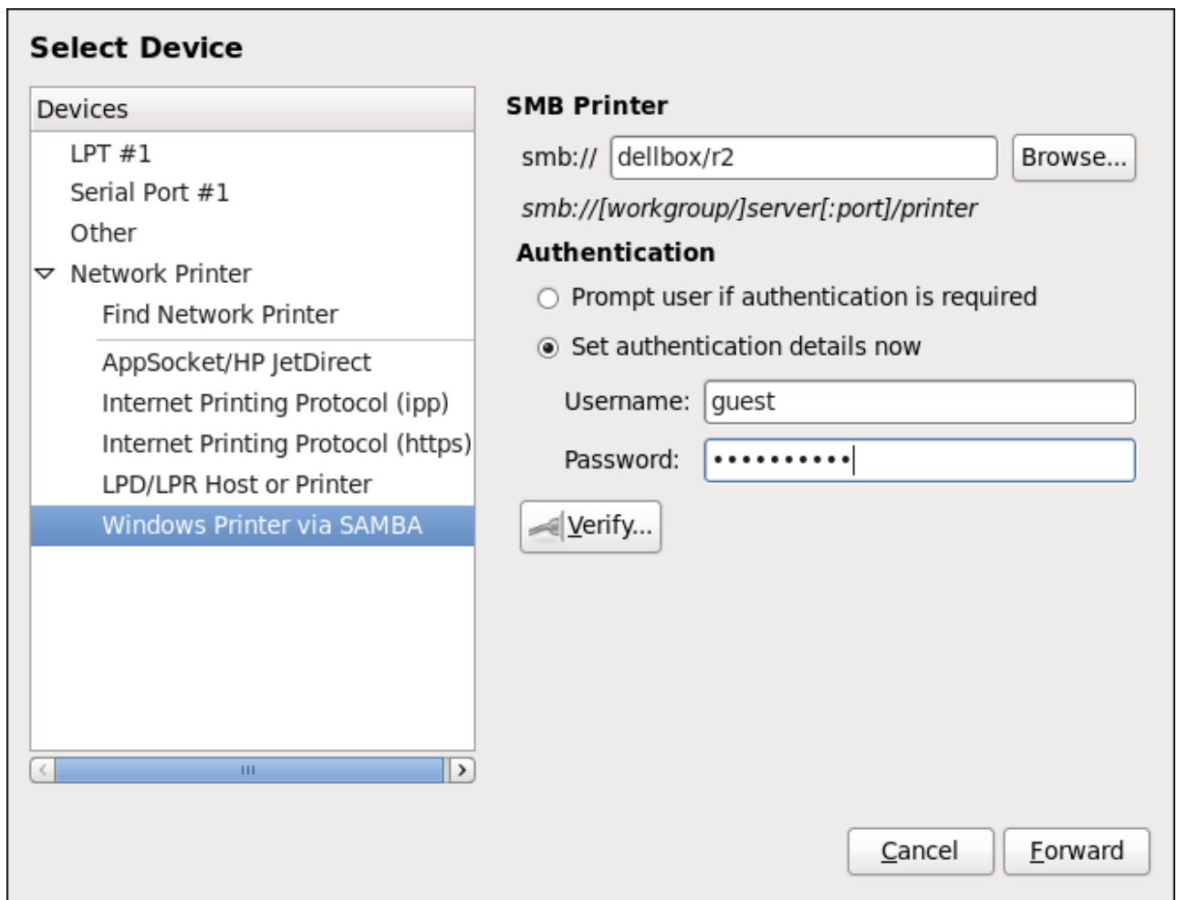
Figure 12.8. Adding a SMB printer
