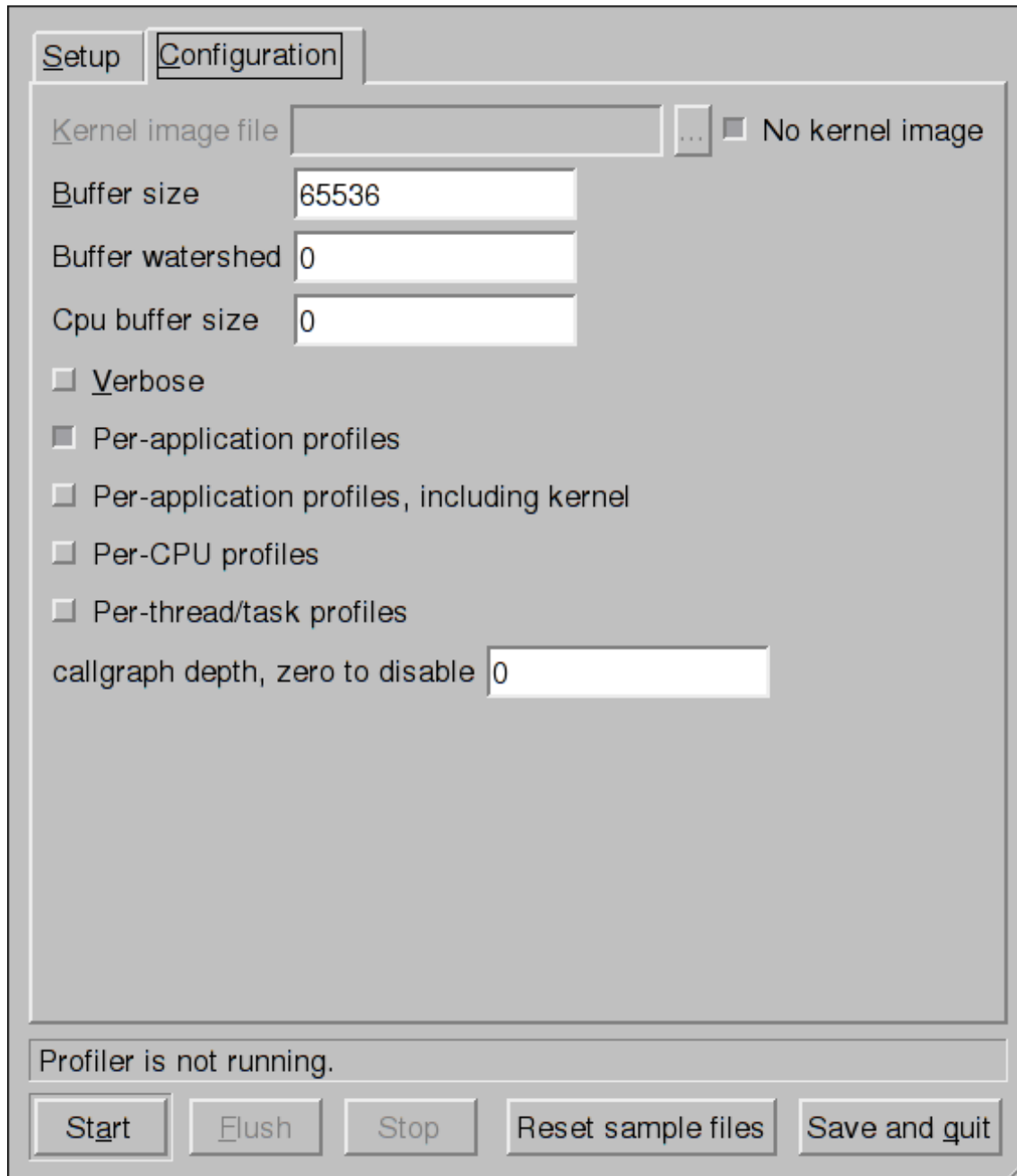
Figure 21.2. OProfile Configuration
