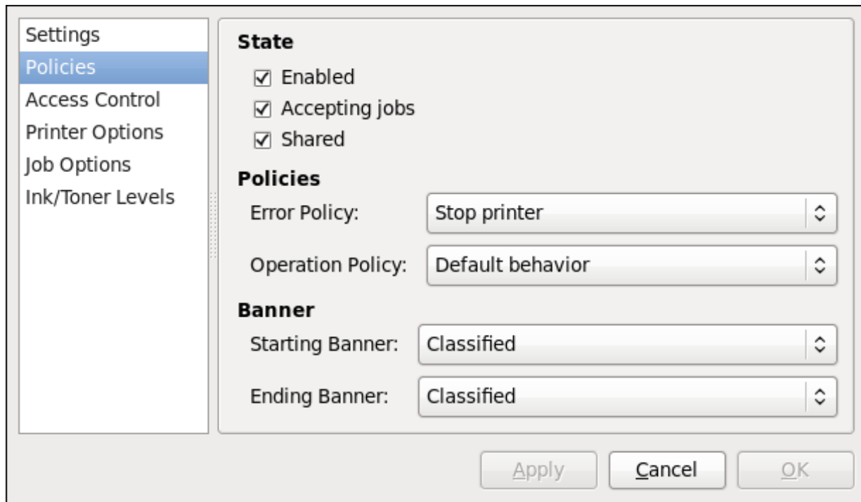
Figure 12.13. Policies page
