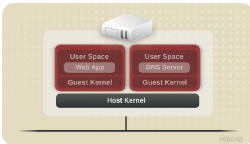
Figure 1.2. Virtualized Environment
